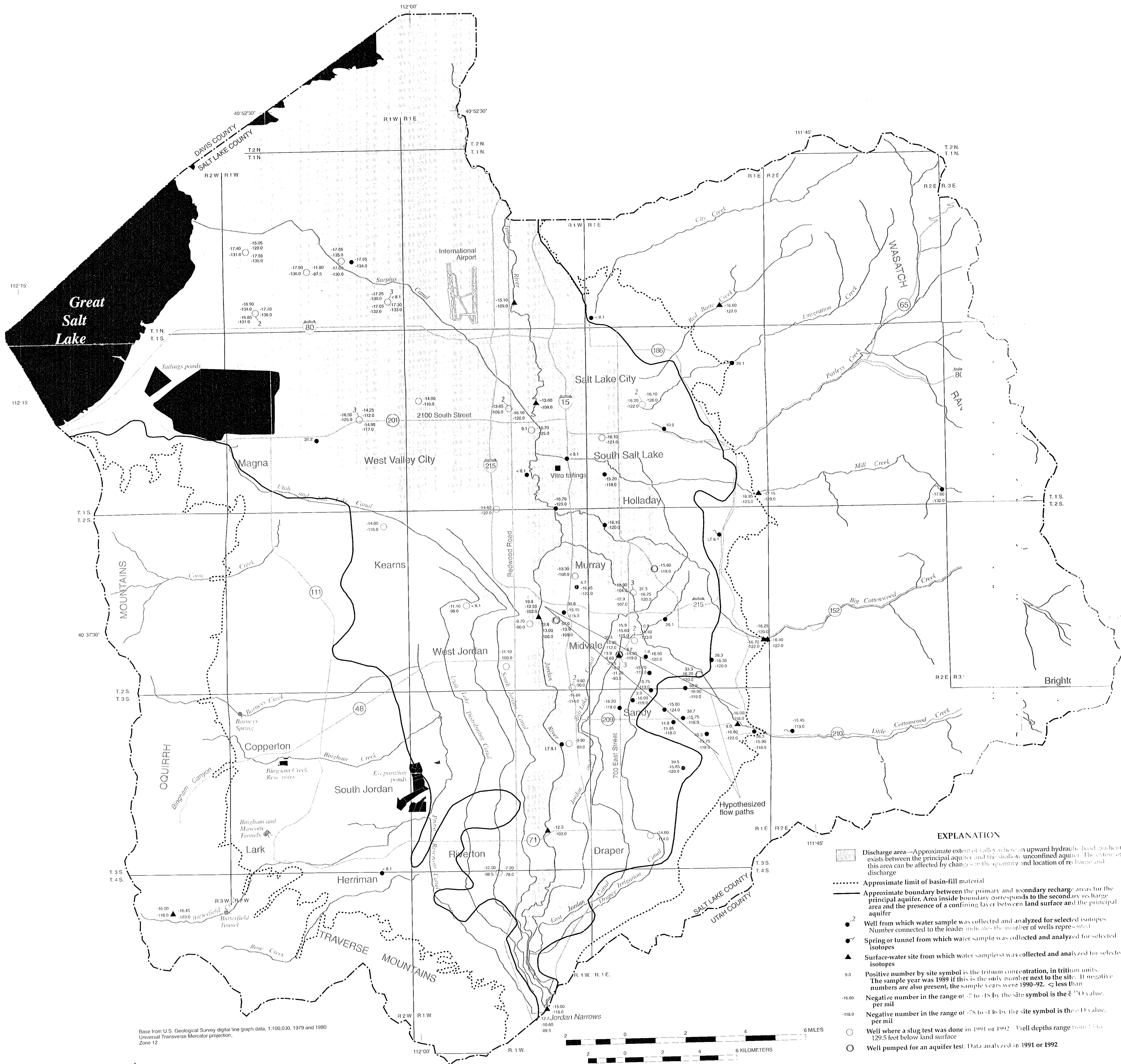
Map showing location of hydrologic-data sites where isotopic data are available; tritium, \delta^{18}\text{O} , and \delta\text{D} values for water samples from selected hydrologic-data sites; and location of wells where a slug test or aquifer test was done; Salt Lake Valley, Utah, 1990–92
