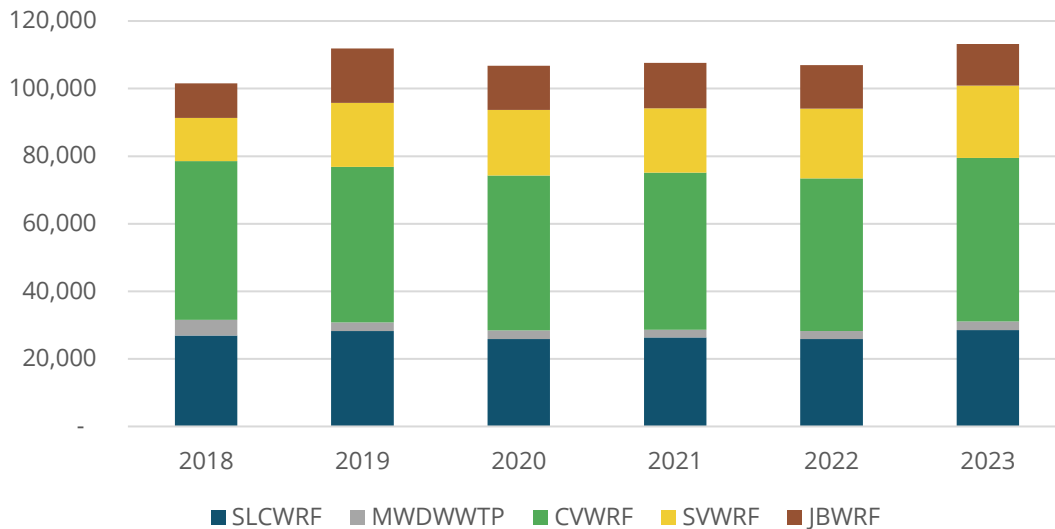
Figure 2. Return Flow (I&I Removed) Total Volume (Acre-Feet)
