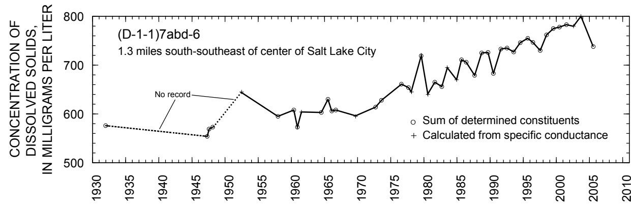
Figure 10. Relation of water level in selected wells completed in the principal aquifer in Salt Lake Valley to cumulative departure from average annual precipitation at Silver Lake near Brighton, and relation of water level in well (D-1-1)7abd-6 to concentration of chloride and dissolved solids in water from the well—Continued.
